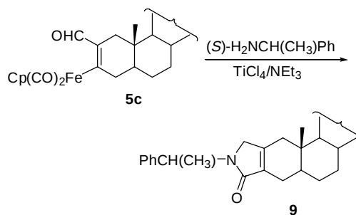
Scheme 2 Synthesis of the \alpha,\beta -unsaturated \gamma -lactam 9
