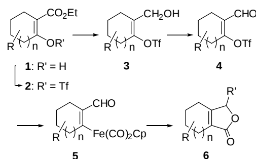
Scheme 1 Synthesis of \alpha,\beta -butenolides from iron-substituted enals derived from \beta -keto esters
